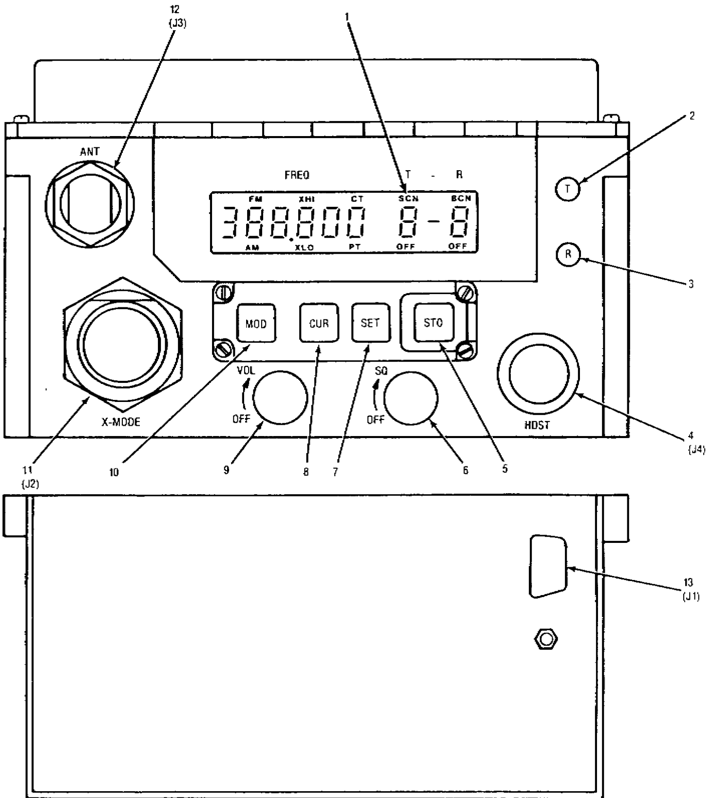
Figure 2-1. Front Panel Controls, Indicators and Connectors
