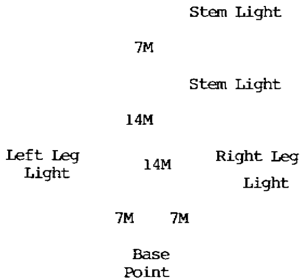
Figure 3-9. Inverted Y.
