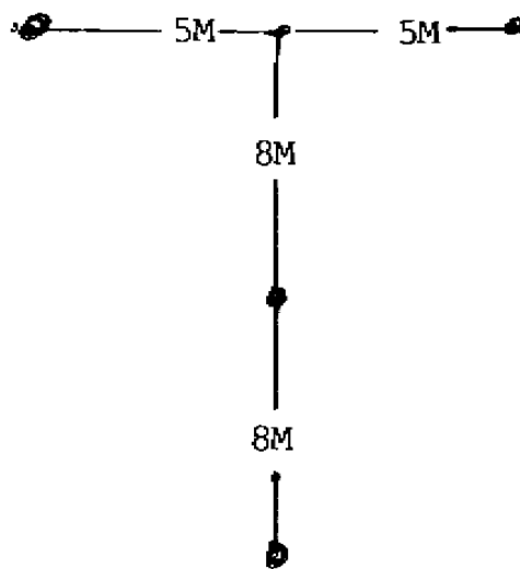
Figure 3-12.1 VAPI when used with T (cargo aircraft).
