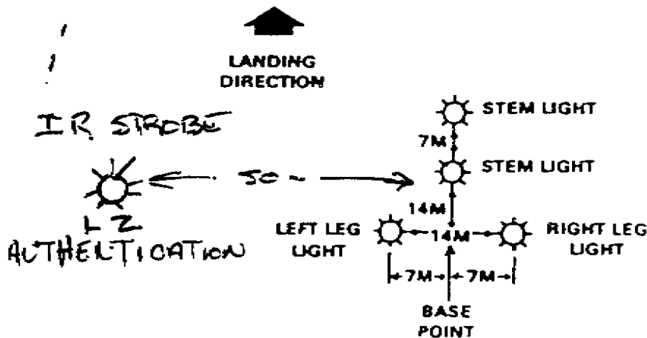
Figure 3-9. Inverted Y.
